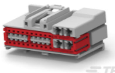
TE Part # 1-2236269-2 24POS, MIXED,REC HSG, 20GENYMCP,ASSY,CODB
